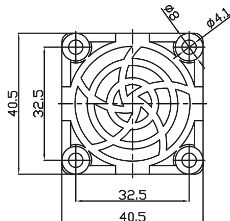
LOWER HOUSING
