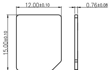
Micro SIM
