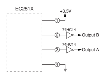
EXTERNAL CIRCUIT
