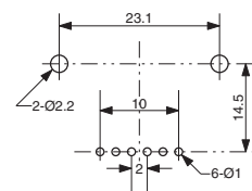
PCB Footprint
