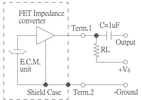
Schematic Diagram
