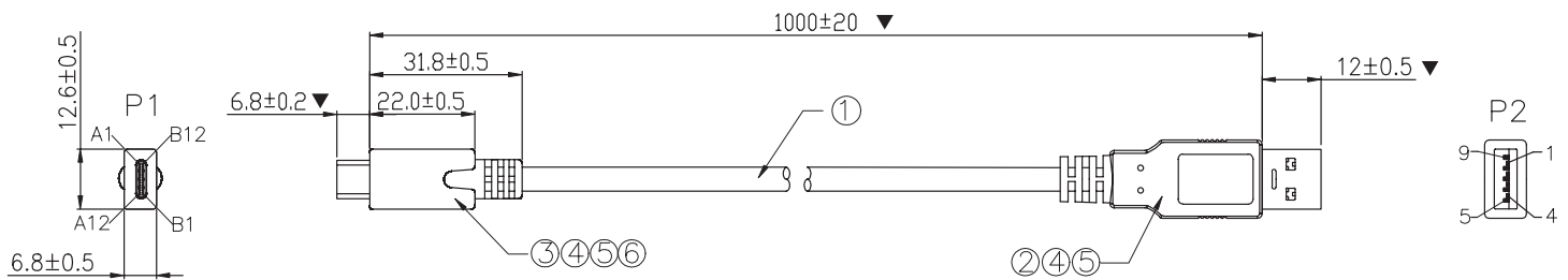
WIRING DIAGRAM
