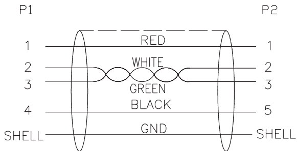
PIN Assignment
