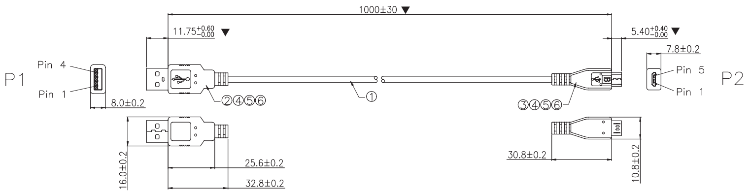
PIN Assignment
