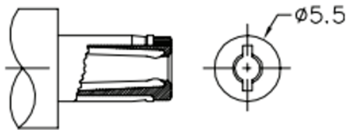
MATING PLUG Jack Insertion Depth: 9.15 mm
