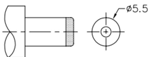
MATING PLUG Jack Insertion Depth: 8.5 mm
